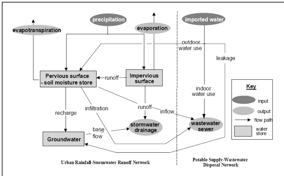
Figure 4 The urban water system as represented by Aquacycle
