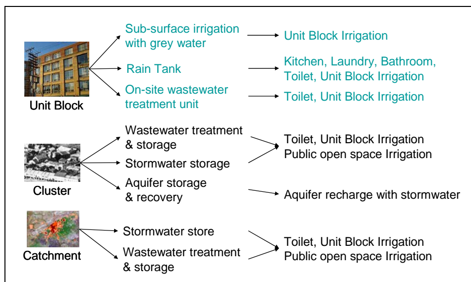
Figure 5 Alternative recycling and reuse schemes at Unit Block, Cluster and Catchment scale levels
