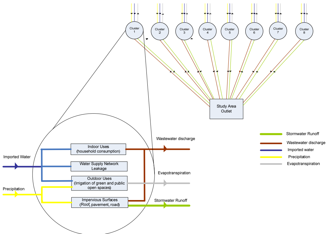
Figure 8 Conceptual representation of the urban water system
